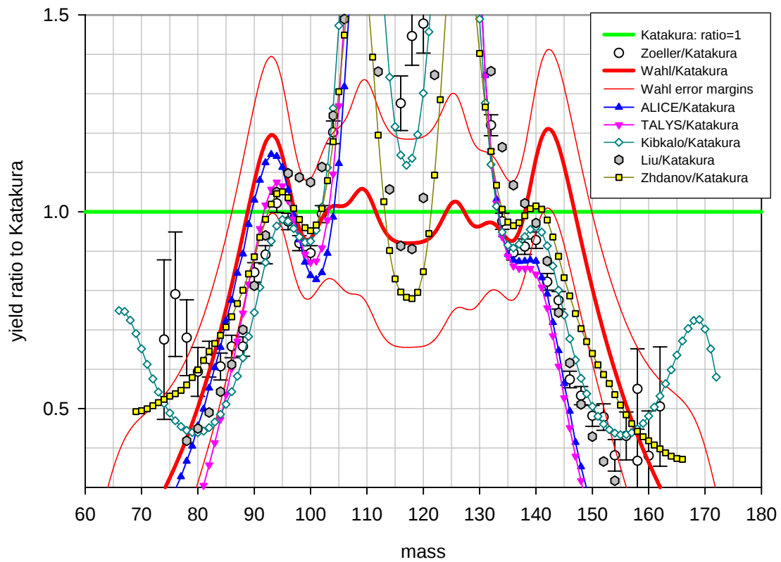
Benchmark A: ^{238}\text{U} around 13 MeV, post neutron emission yield ratio to Katakura's systematics lower graph: partial plot (very high and low values omitted).
